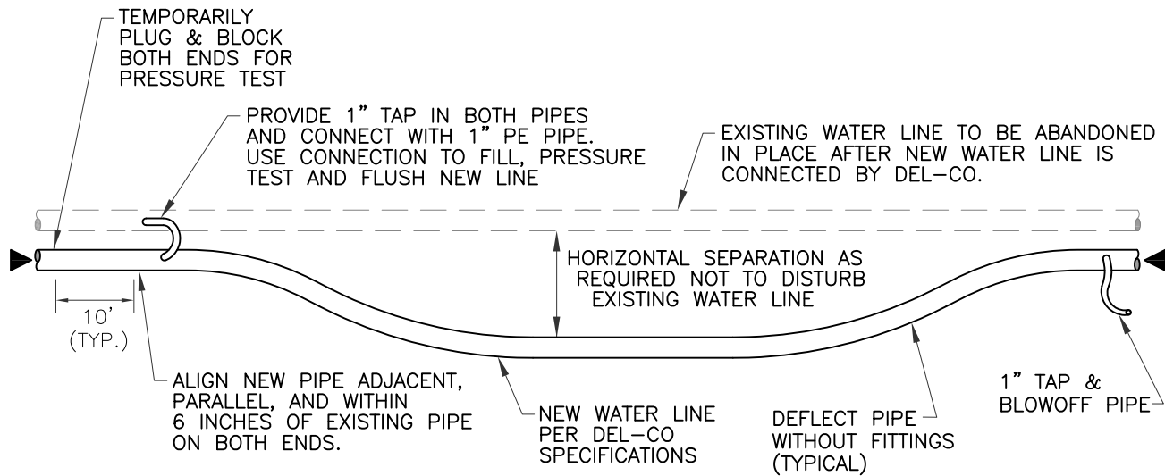
PLAN NTS
